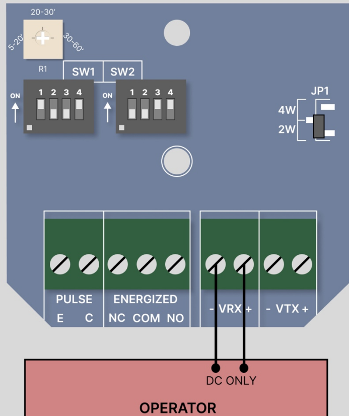
Wiring Diagram D: Two-Wire Pulse (2 Frequency: 300Hz, 0Hz)
