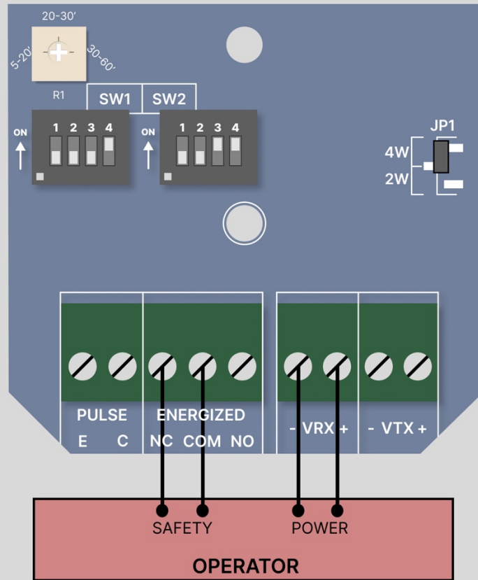
Wiring Diagram A: Normally Closed
