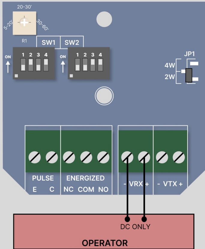
Wiring Diagram E: Two-Wire Pulse (3 Frequency: 300Hz, 2Hz, 0Hz)
