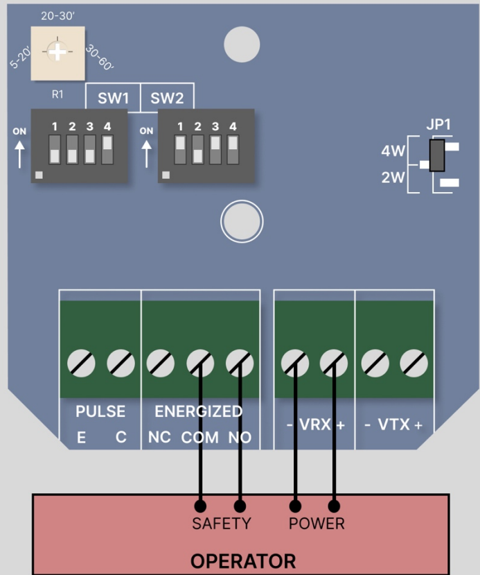
Wiring Diagram B: 10K Resistive Termination
