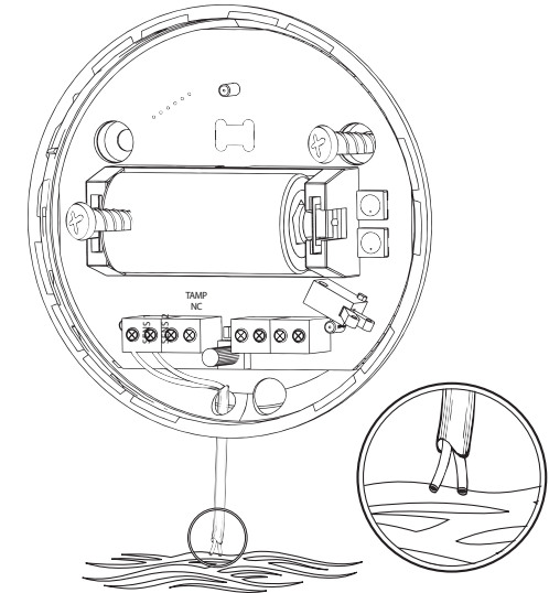
Fig. 3 - Flood sensor's contacts extended with a wire
