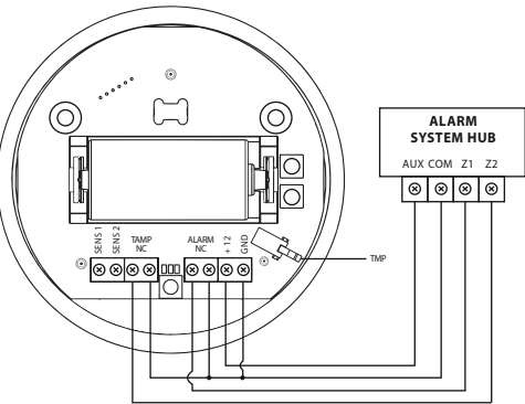
Fig. 1 - Connection with alarm system
